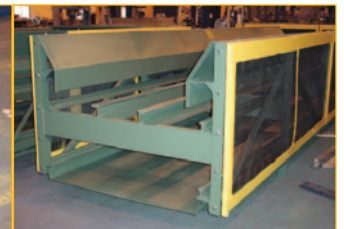
Open frame with flared 18" high skirting and 2 load impact rails
